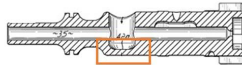
Battle Bolt™ cross section
