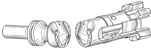
Battle Bolt™ cut-away
